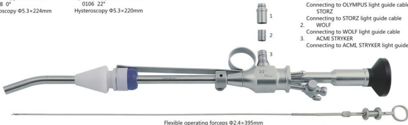
Flexible operating forceps \Phi 2.4 \times 395\text{mm}
